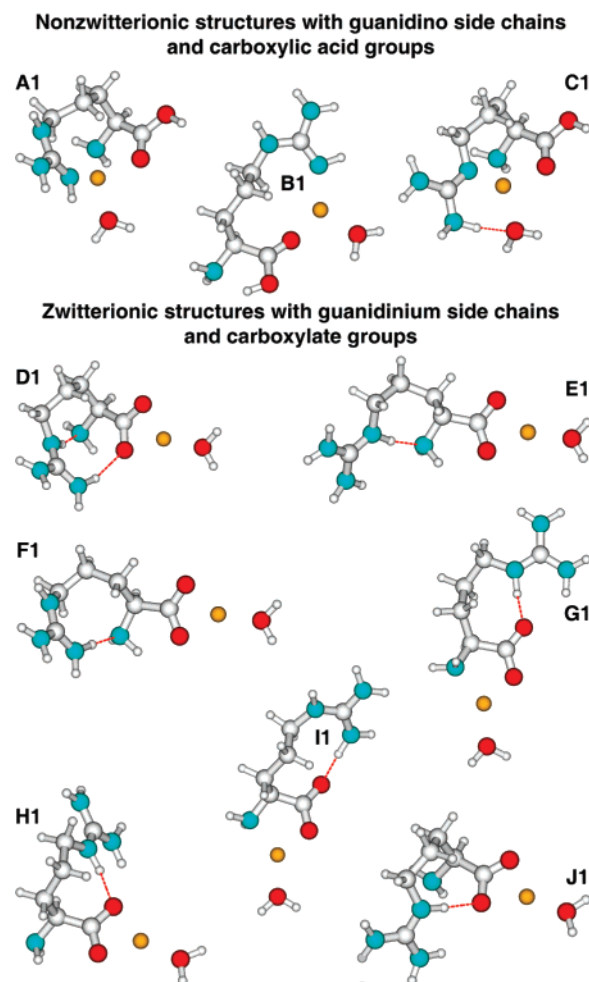
Figure 2. Energy minimized structures A1 – J1 of the nonzwitterionic and zwitterionic forms of Arg•Li + (H 2 O) from B3LYP/6-31++G** calculations.
