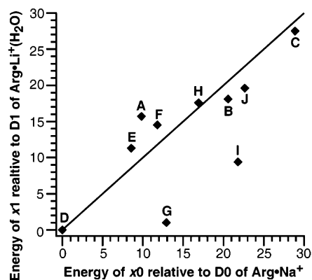
Figure 7. The B3LYP/6-31++G** energies (in kJ/mol, including zero-point energies) of the x1 , x = A-J , structures of \text{Arg}\cdot\text{Li}^+(\text{H}_2\text{O}) plotted versus those of the corresponding x0 structures of \text{Arg}\cdot\text{Na}^+ . The plotted line has a slope of unity.
