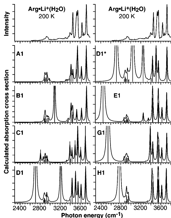
Figure 5. Photodissociation spectrum of \text{Arg}\cdot\text{Li}^+(\text{H}_2\text{O}) and B3LYP/6-31++G** calculated spectra for selected conformers of this ion. The intensities of the calculated spectra are scaled to the higher-frequency bands in the spectra. Un-normalized spectra and additional calculated spectra are shown in Supporting Information Figure 5–7.
